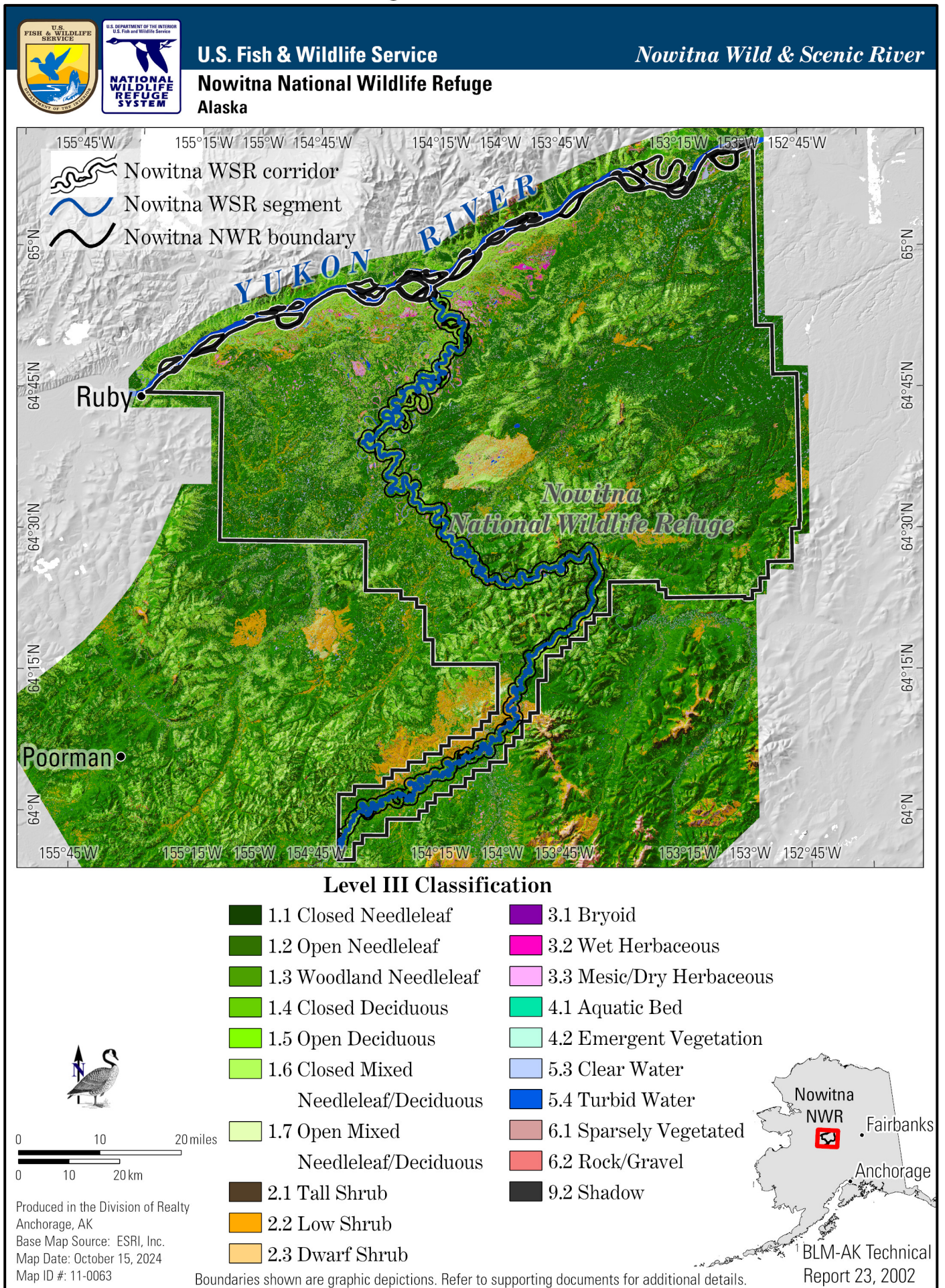
Figure 5: Land Cover 1
