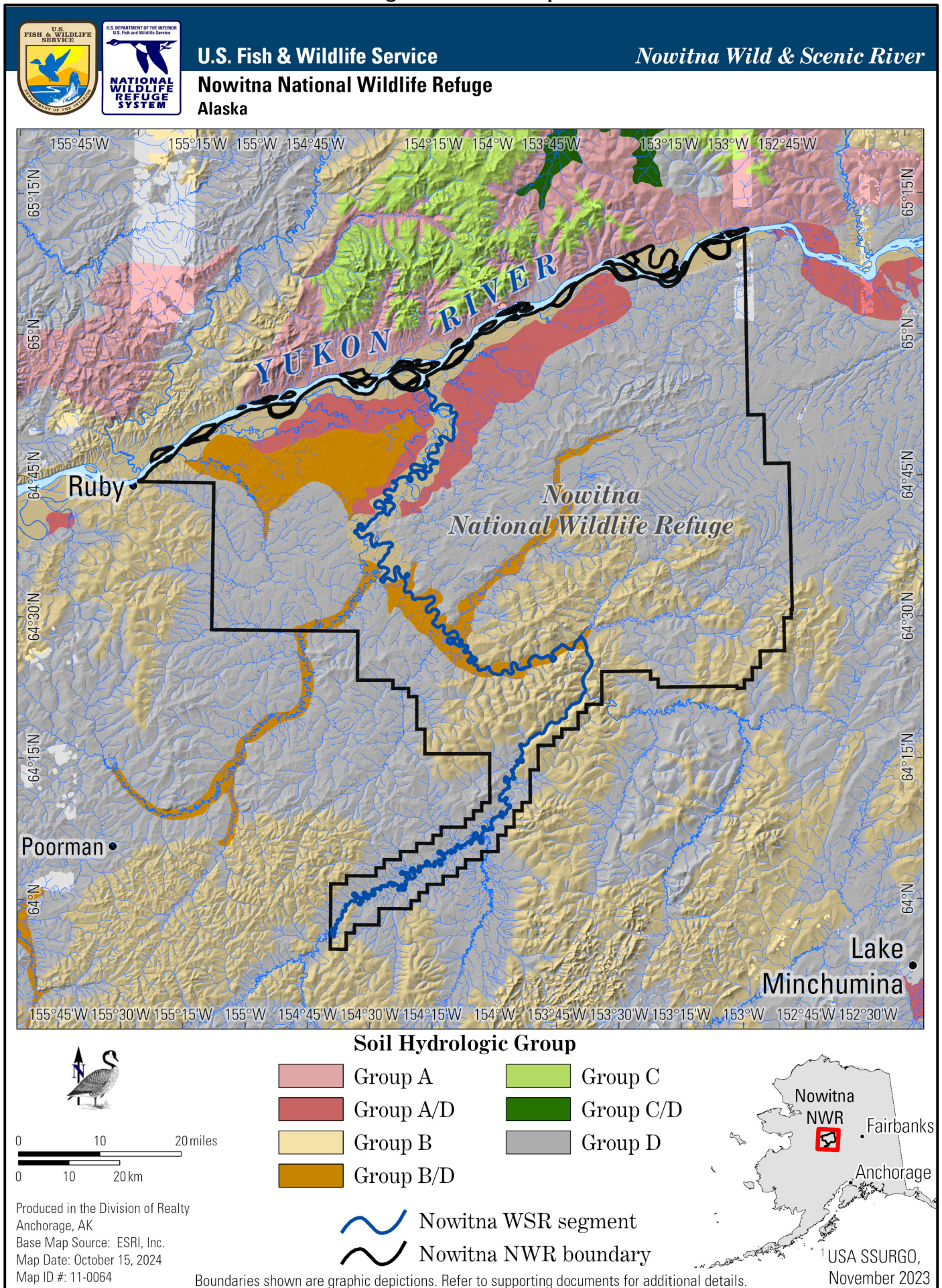
Figure 9: Soil Groups 1
